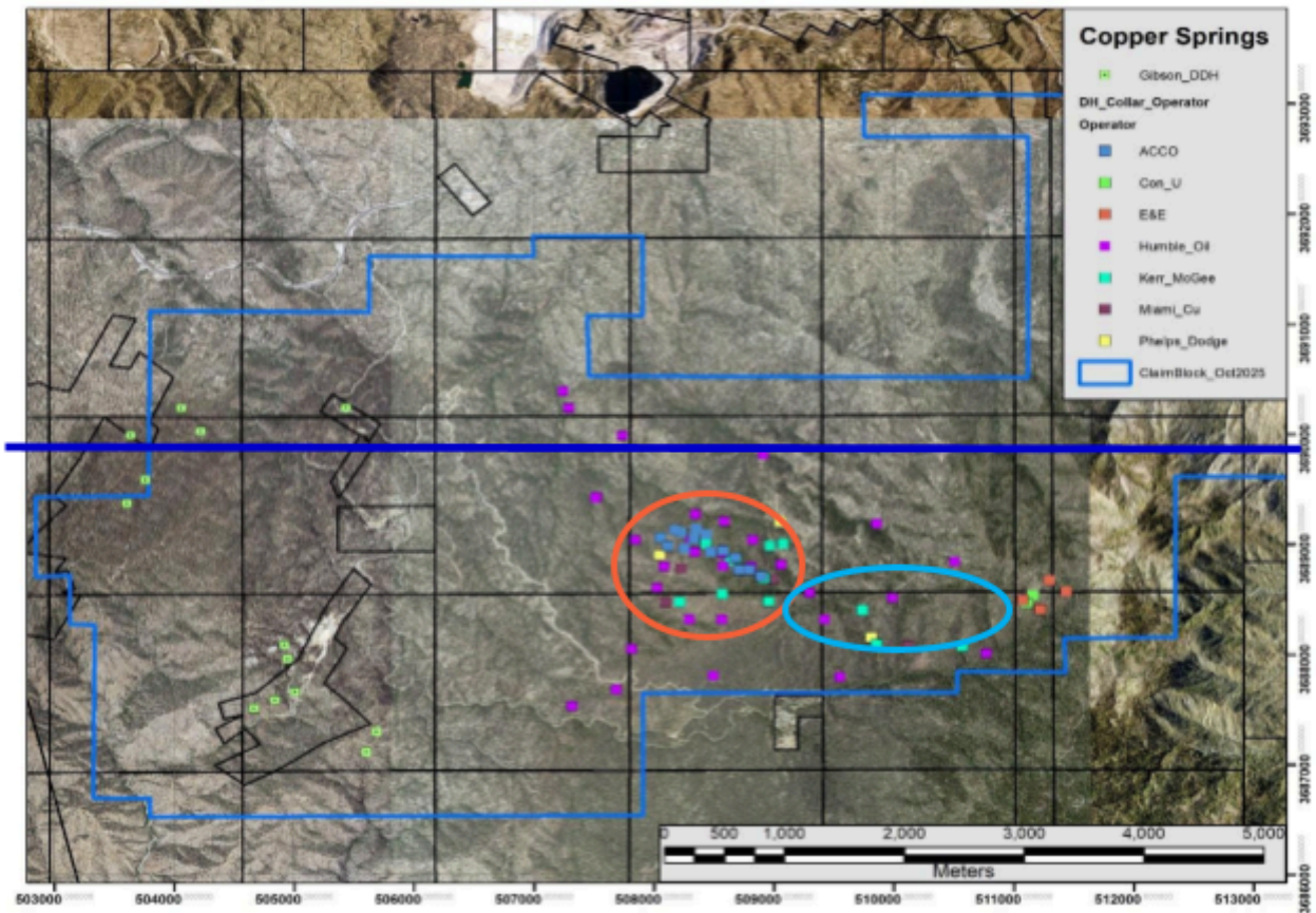
Figure 9.1.1 Project Map showing Drill Hole Locations by Company. The West Lobe and East Lobe are indicated by red and blue polygons. Section Line of Figure 9.1.4 concept is shown by dark blue line.
