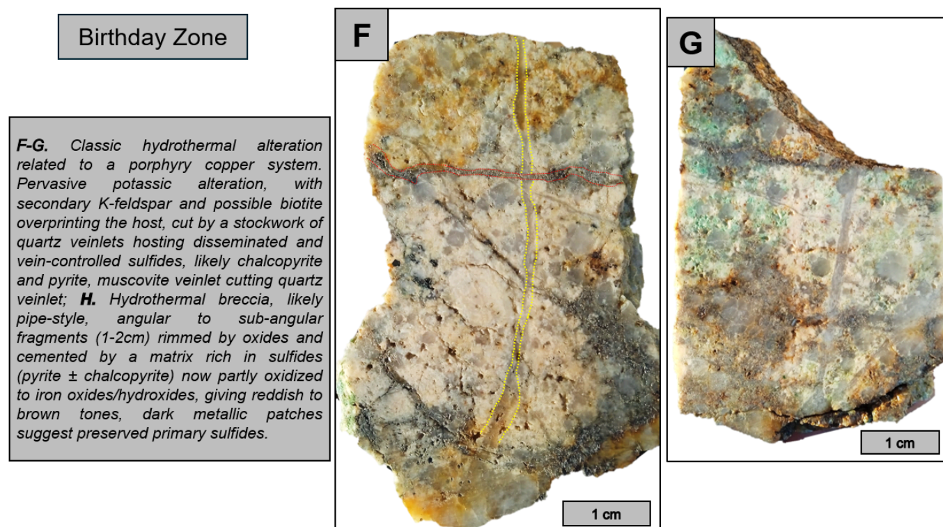
Figure 7.5.2 Birthday Zone Alteration Examples- F) pervasive potassic alteration w secondary K-Feldspar and possible biotite;
