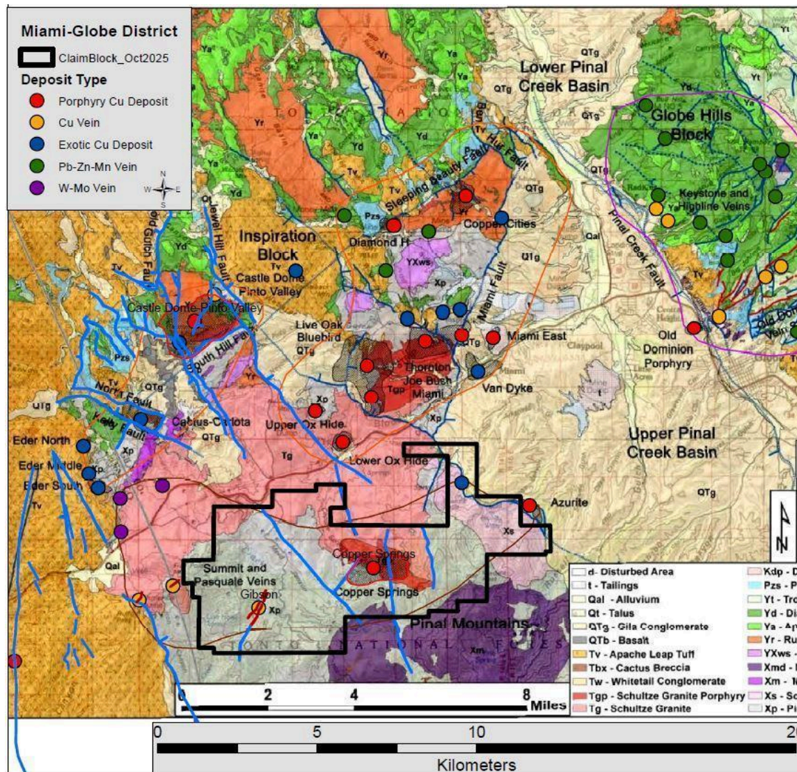
Figure 7.0.1 Regional Geologic Map showing mineralization. The Property is indicated by the black outline.
