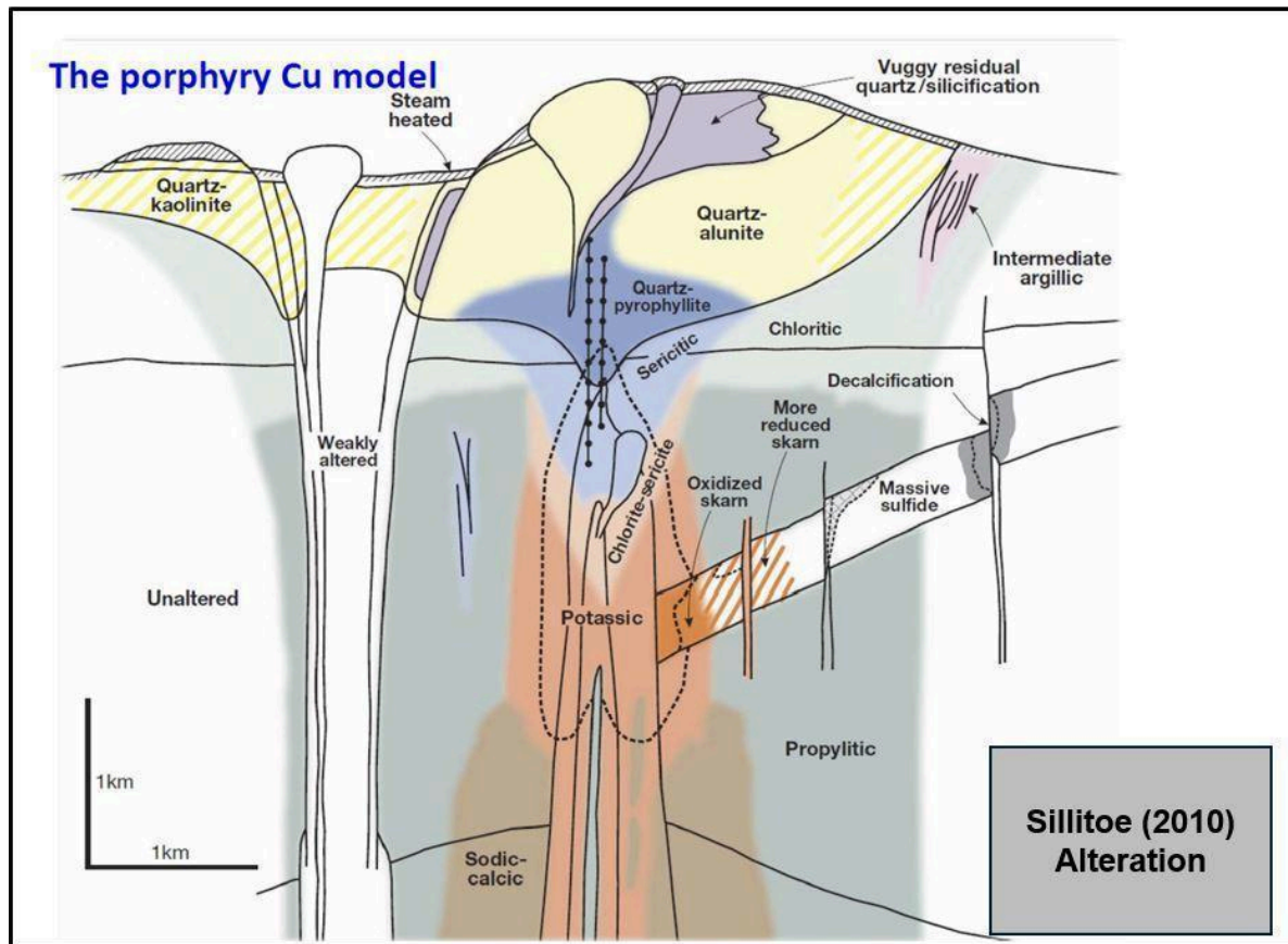
Figure 8.0.1. Idealized Model for the Classic Porphyry Copper Deposit, from Sillitoe, 2010.
