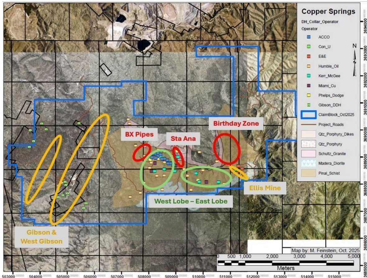
Figure 6.2.1 Project Map with target zones indicated by colored ellipses; red is hypogene porphyry mineralization, green are exotic copper mineralization, orange are mineralized veins/shears. Section Line of Figure 6.1.4 concept is shown by black line.
