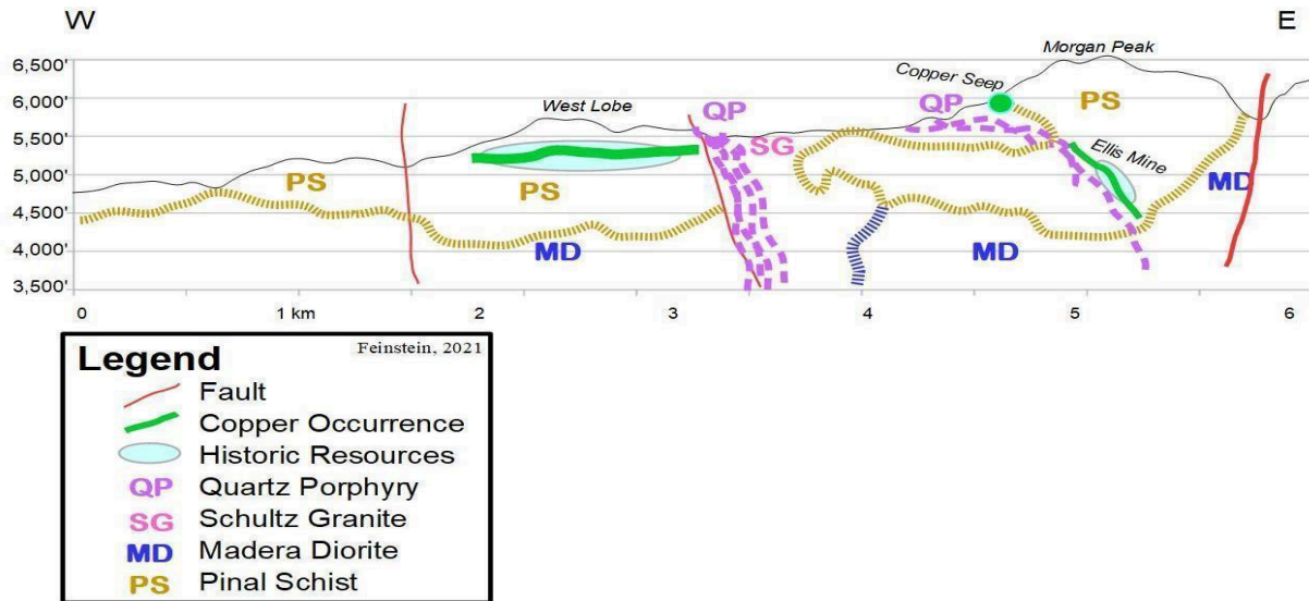
Figure 9.1.4 Copper Springs Conceptual Section
