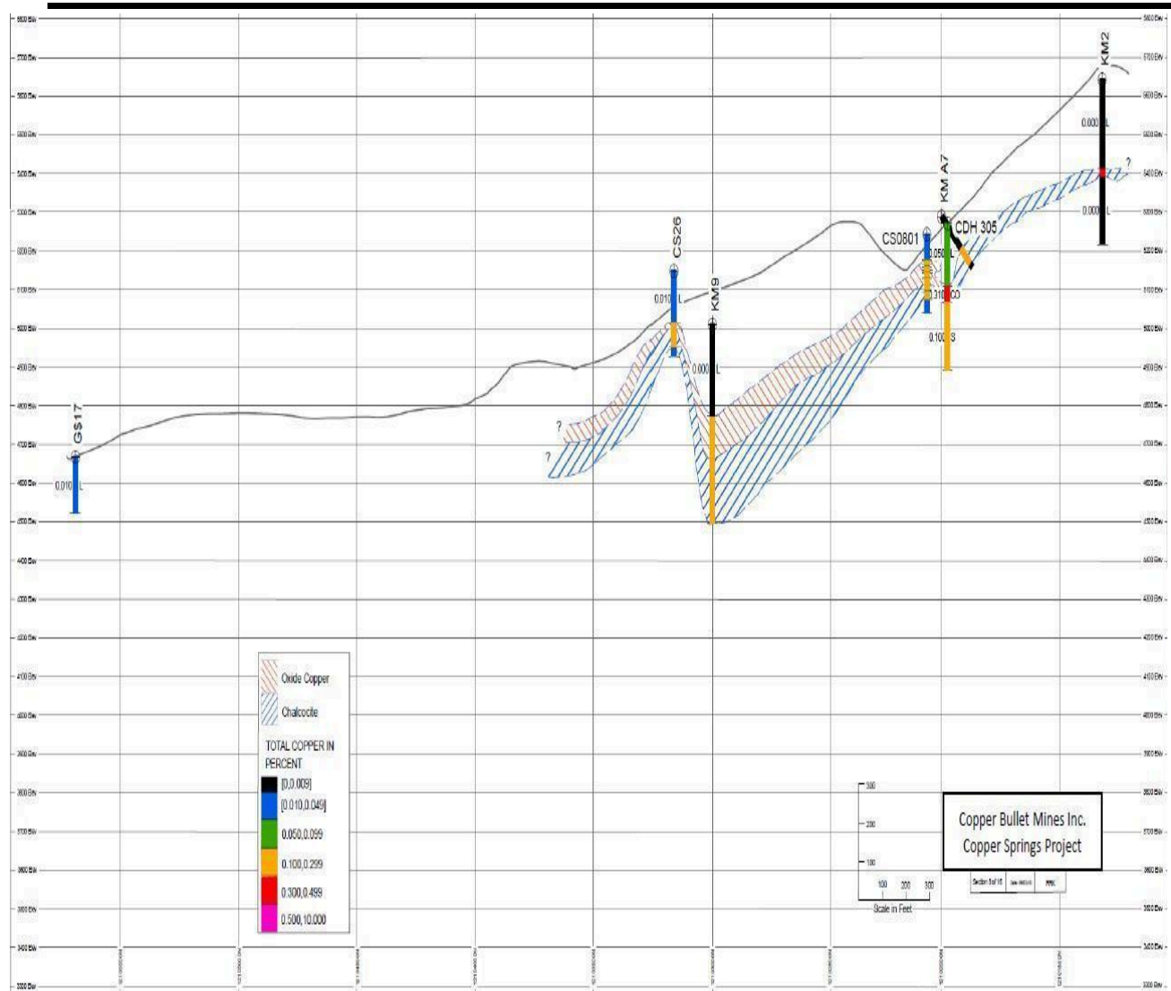
Figure 6.6.3 Cross-Section #8, Toro Resources, 2010
