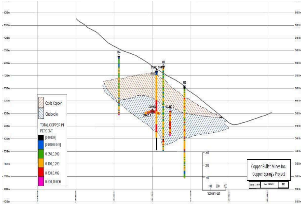
Figure 6.6.2 Cross-Section #13, Toro Resources, 2010.
