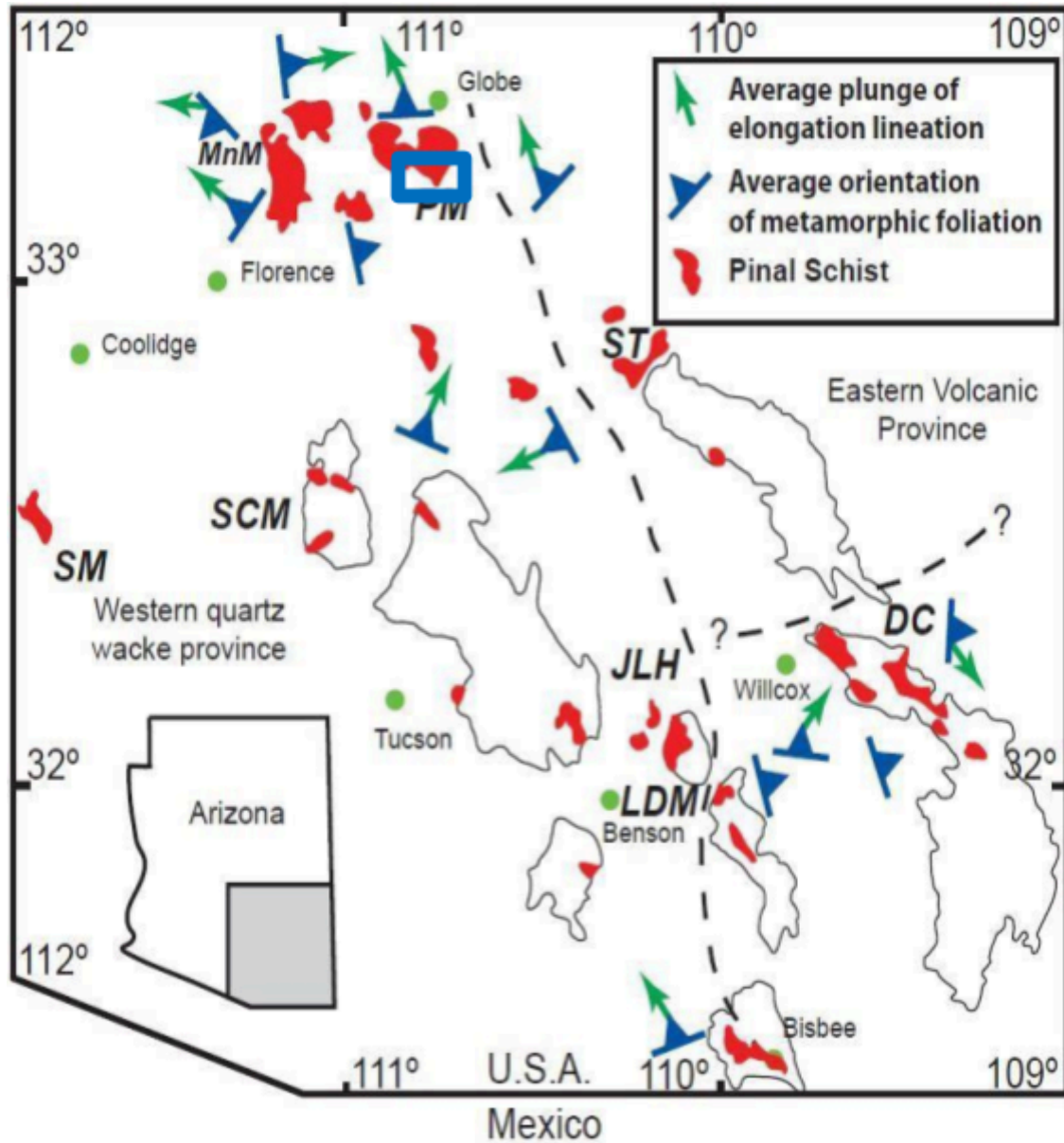
Figure 7.3.1.1 Distribution of the Pinal Schist in southeast Arizona. Copper Springs project indicated by blue rectangle (modified from Doe, 2014).
