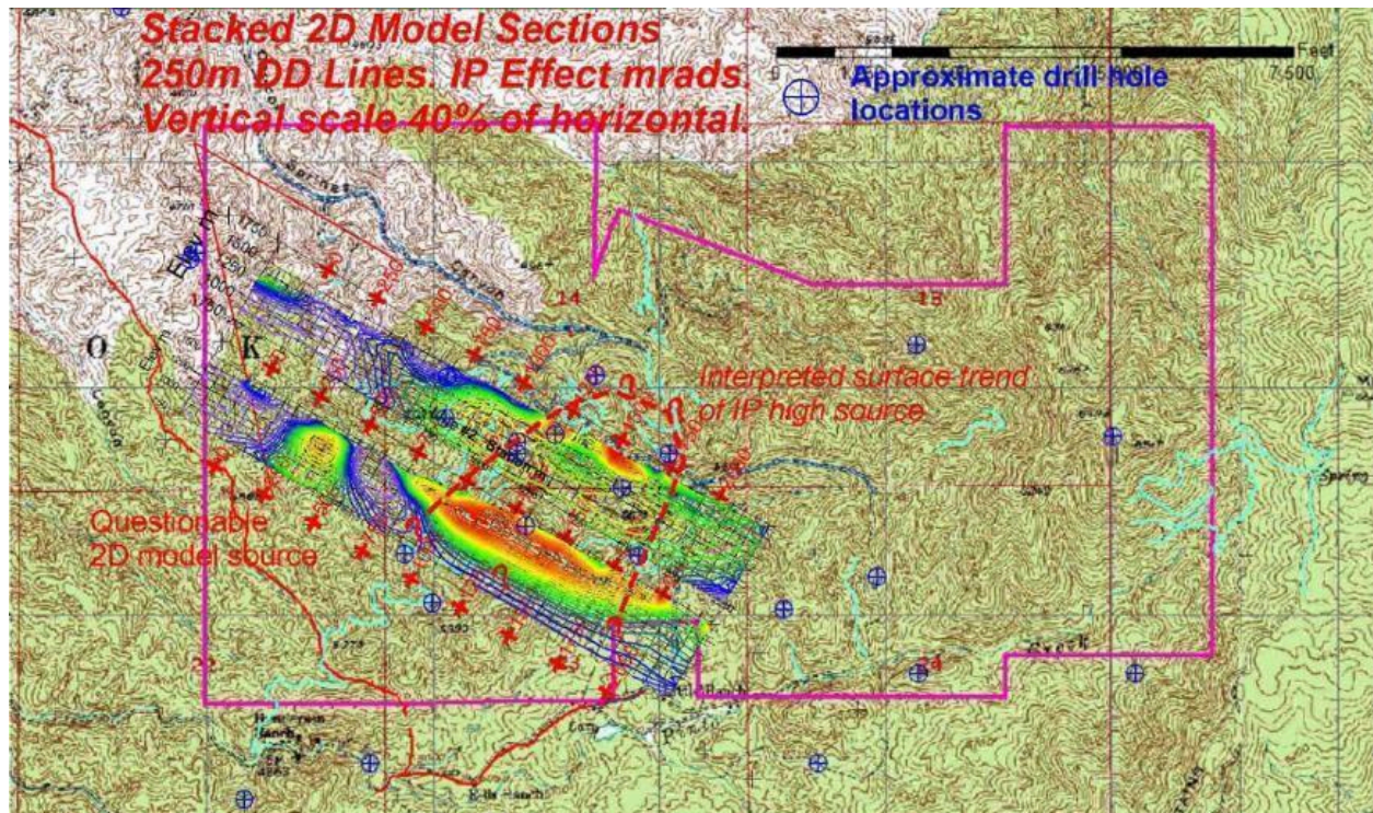
Figure 6.4.1 2007 IP geophysical survey shown on Topographic map.
