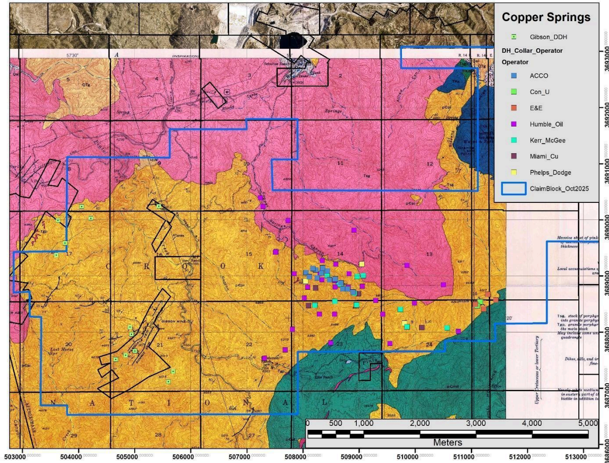
Figure 7.3.2.1 The Copper Springs Property with geology and drill-holes by operator shown. Santa Ana Shear Zone shown in red.
