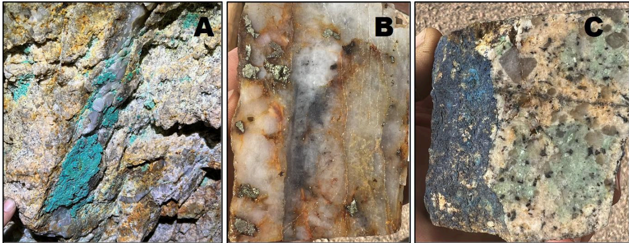
Figure 7.4.1 Mineralization observed in Santa Ana Tunnel. A) Abundant copper oxides and strong quartz-chalco-moly vein stockwork; B) Sheeted quartz vein with coarse euhedral chalcopyrite and zones of fine CCPY+MOLY; C) Quartz porphyry with disseminated chalcopyrite and sulfide veinlets.
