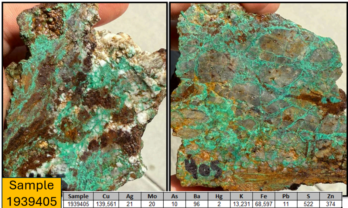
Figure 9.2.3 Rock Sample Photos from the West Gibson Target where high-grade copper results were confirmed. Left photo shows coarse porphyritic dike with euhedral oxidized chalcopyrite; right photo shows shattered and silicified pinal schist with abundant malachite.
