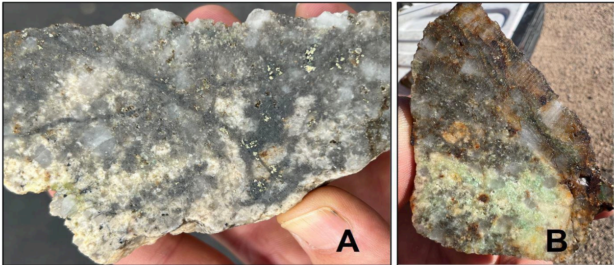
Figure 7.5.1 Examples of Potassic alteration. A) disseminated chalcopyrite with quartz-sulfide stockwork (hypogene); B) copper oxides disseminated in potassic margin of QSP vein (supergene).
