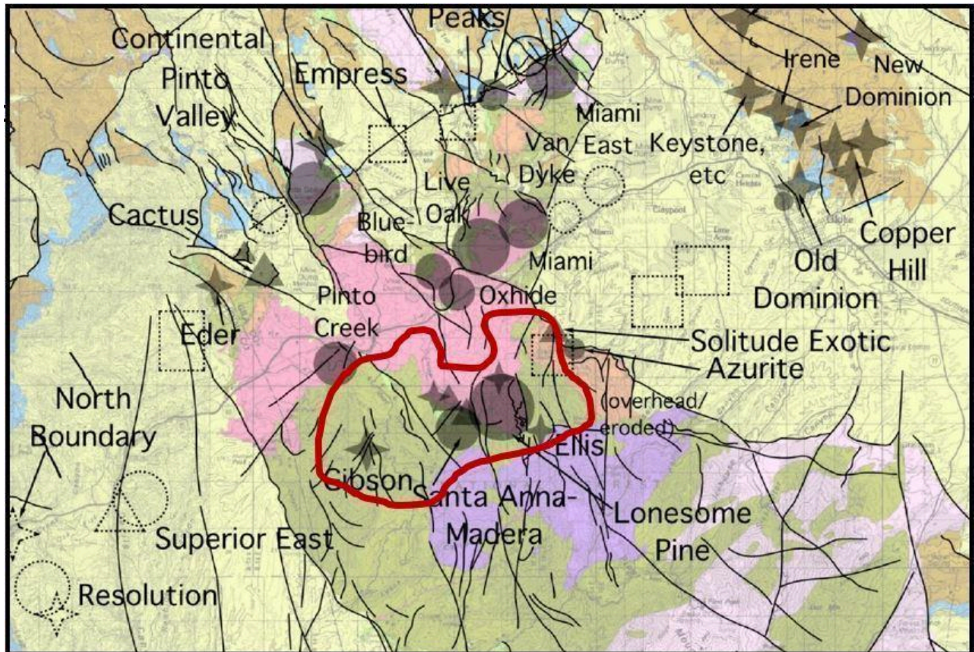
Figure 6.1.1 Interpretive Geologic Map of the Miami-Globe Mining District, from Briggs 2022. The Copper Spring Project is roughly outlined in red. Mineralized bodies are indicated by stars (veins), circle (porphyry intrusion), and triangles (exotic style); the graduated sizes correspond to volumes.
