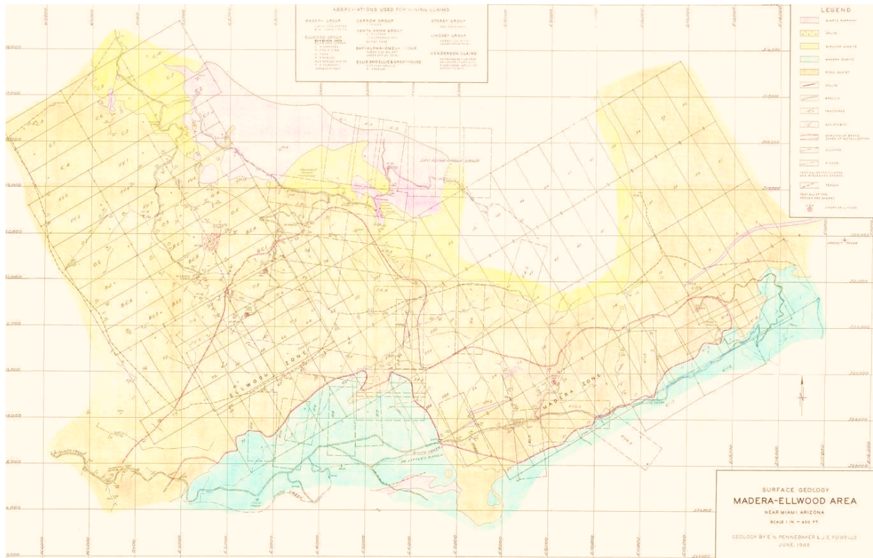
Figure 6.2.2 Geologic Map of the Copper Springs Project, named Madera-Ellwood Area at the time. Mapped by E.N. Pennebaker and J.E. Fowells, June 1948.
