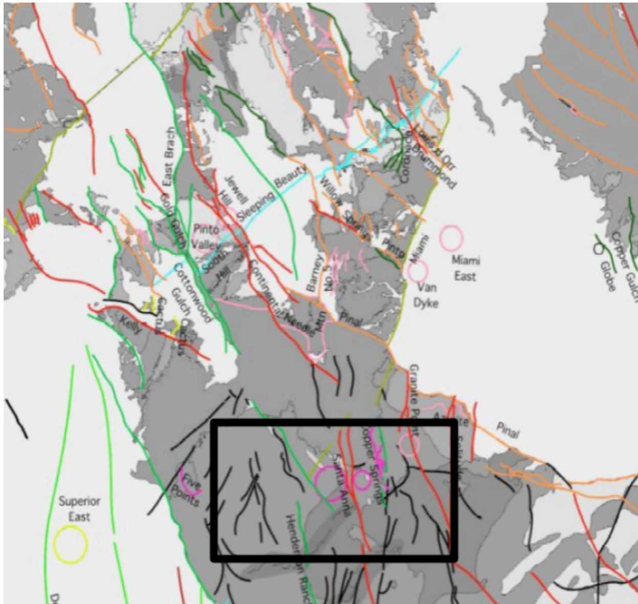
Figure 7.3.3.2 Regional structural map showing the Copper Springs Project in black. Ages of structures are indicated by the colored lines (modified from Maher, 2008).
