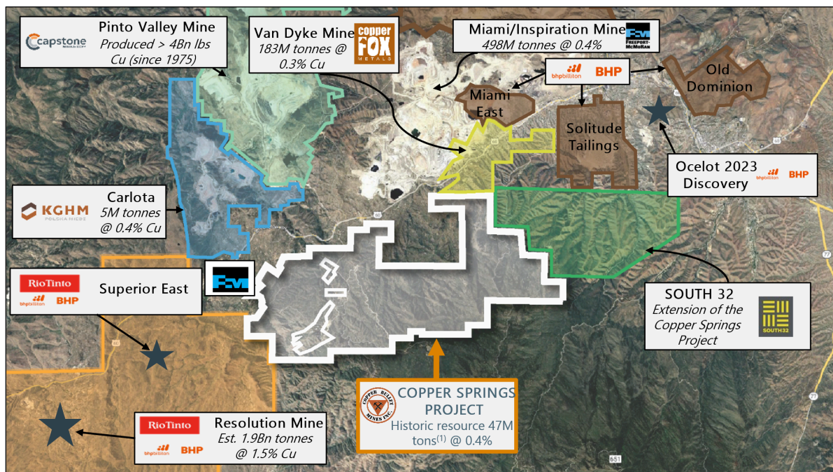
Figure 15.0.1 Copper Springs Location Map with Nearby Mines and Deposits.
