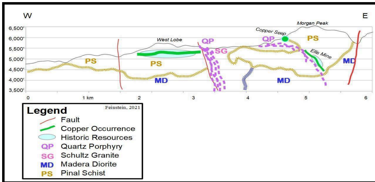
Figure 6.3.3 Copper Springs Conceptual Section.
