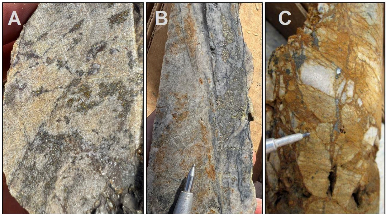
Figure 17.0.1 Sulfide Mineralization on the Copper Springs Project is indicative there may be potential for additional mineralization at depth. A) Chalcopyrite with Bornite (CS-08-02 @ 283ft); B) Qtz+Pyr+Moly Vein (CS-08-03 @ 136ft); C) Coarse Chalcocite in Breccia (CS-08-04 @ 158ft).
