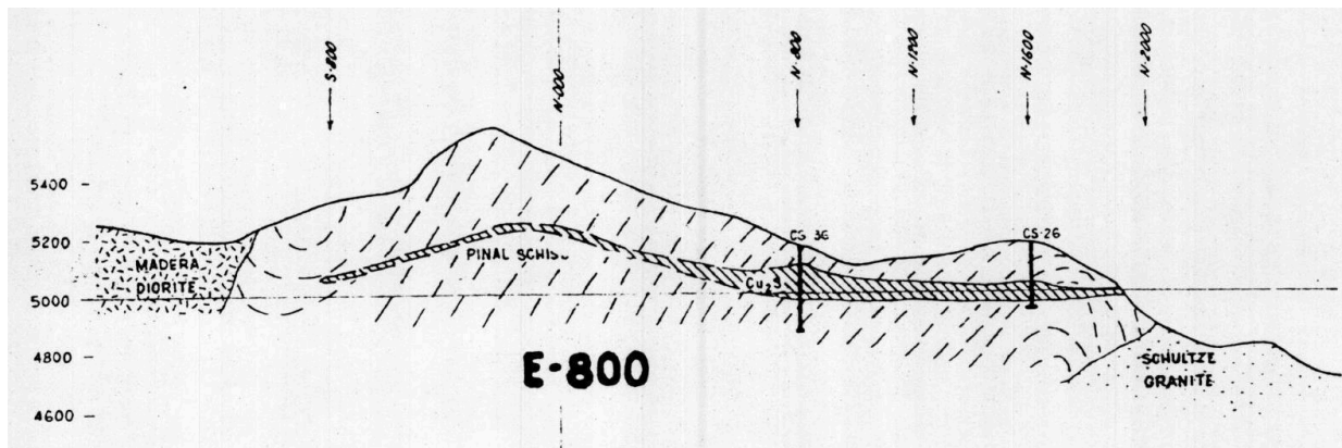
Humble Oil South-North Section Line E-800- This section depicts the supergene blanket of interest.
