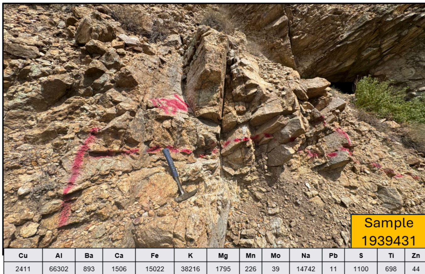
Figure 9.2.2 Outcrop photo of sample 1939431, 1.6m, with geochemical sample results in chart.
