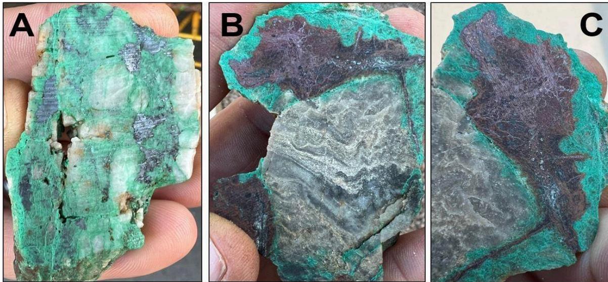
Figure 9.1.3 Rock Samples collected from Ellis Mine representing the brittle portion of a mineralized shear zone. A) Sheeted quartz veins with coarse euhedral bornite; B+C) Chrysocolla cemented breccia shows a shear-deformed clast rimmed by bornite and cuprite with native copper.
